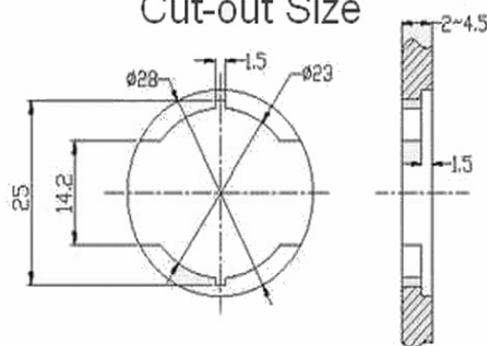
Cut-out Size
